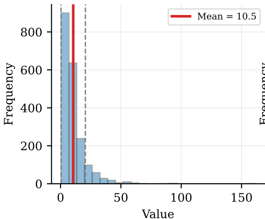
Raw Distribution (skewed)
