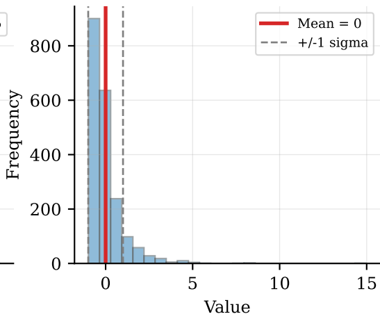
Standardized (mu=0, sigma=1)
